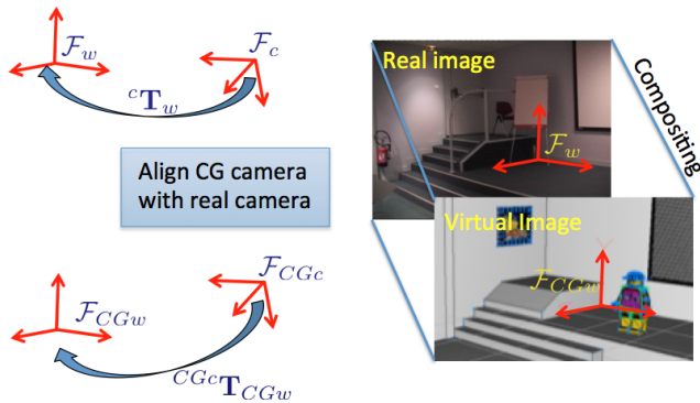
Fig. 1. AR Principle and considered coordinate systems: to achieve a coherent compositing, computer graphics (CG) camera and real one should be located at the very same position and have the same parameters.
